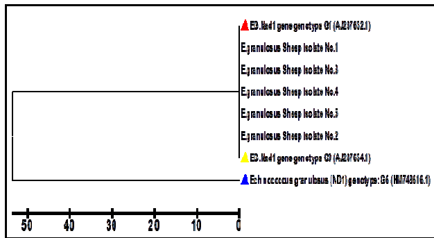
Figure 2: Phylogenetic tree analysis based on nad1 gene partial sequence that used for E. granulosus genotyping detection of sheep isolates. The phylogenetic tree was constructed using Unweighted Pair Group method with Arithmetic Mean (UPGMA tree) in (MEGA 6.0 version).
