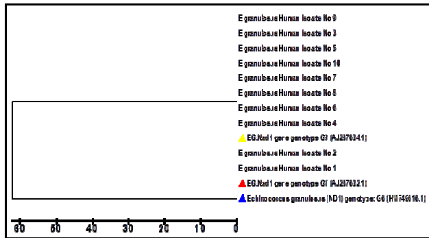
Figure 1: Phylogenetic tree analysis based on nad1 gene partial sequence that used for E. granulosus genotyping detection of human isolates. The phylogenetic tree was constructed using Unweighted Pair Group method with Arithmetic Mean (UPGMA tree) in (MEGA 6.0 version).
