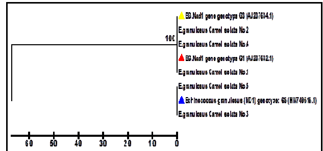
Figure 4: Phylogenetic tree analysis based on nad1 genes partial sequence that used for E. granulosus genotyping detection of camel isolates. The phylogenetic tree was constructed using Unweighted Pair Group method with Arithmetic Mean (UPGMA tree) in (MEGA 6.0 version).
