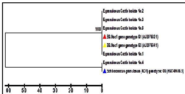
Figure 3: Phylogenetic tree analysis based on nad1 genes partial sequence that used for E. granulosus genotyping detection of cattle isolates. The phylogenetic tree was
